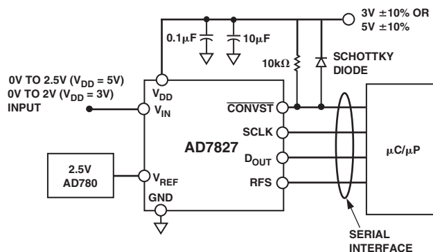
Figure 1. Typical Connection Diagram of the AD7827
